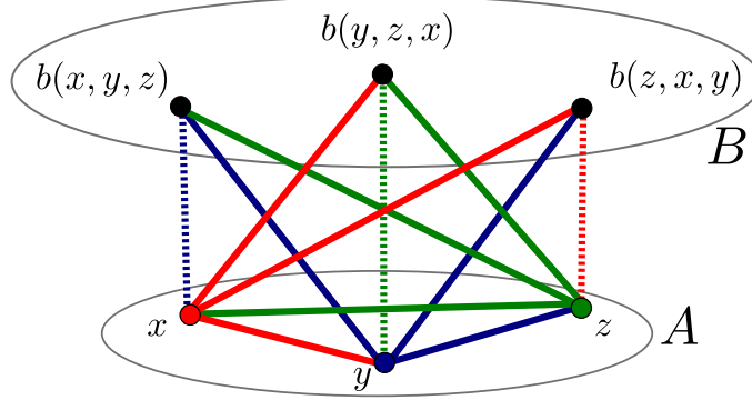
Figure 1: How edges involving x, y, z are distributed between the spiders D_x, D_y, and D_z for a triple (x, y, z) \in \vec{\mathcal{S}} . Here the colours do not correspond to the colours of edges in G , but rather to the three spiders D_x, D_y, and D_z : red edges are in D_x , blue edges are in D_y , and green edges are in D_z . The three dashed edges all have the same colour in G as a consequence of Claim 13 (i).
